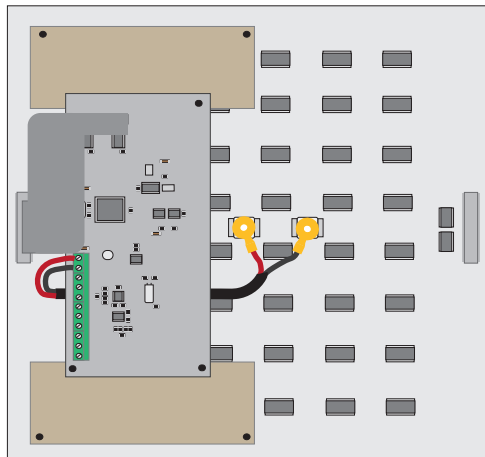
GRGB controller, Connections
